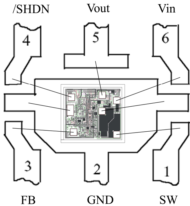
Assembly Drawing SOT-23-6 (bottom view)
