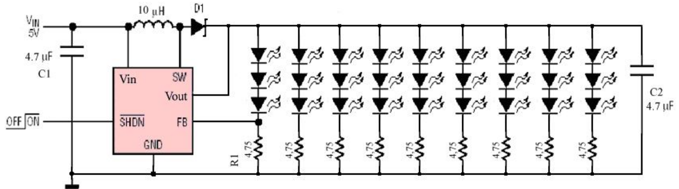
Figure 1. TYPICAL APPLICATION
