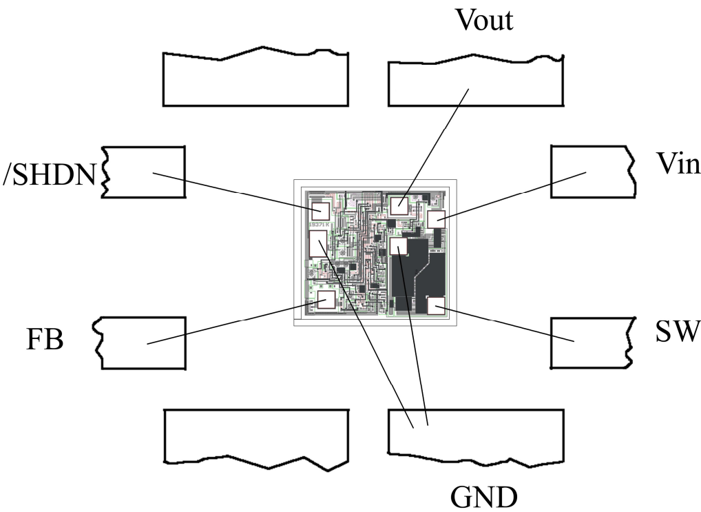
Assembly Drawing SO-8
